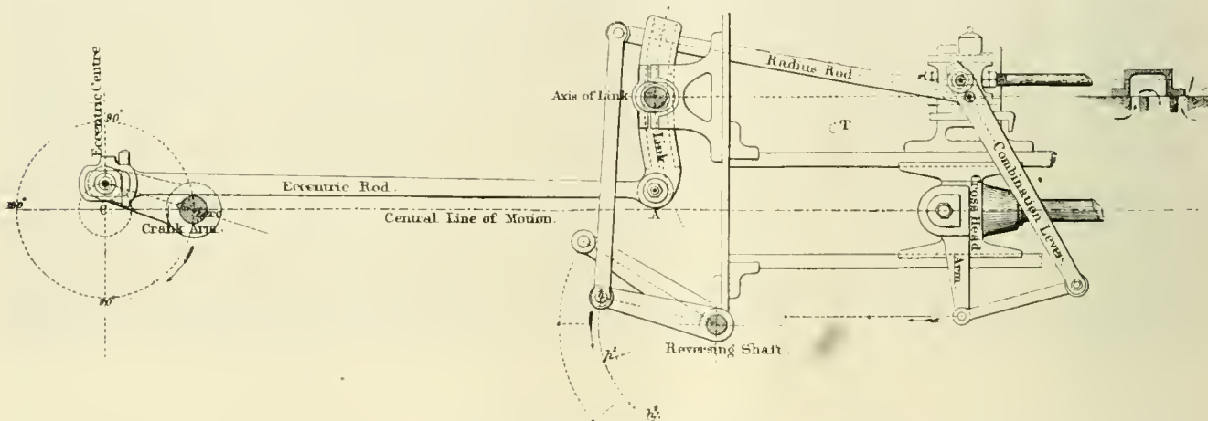
WALSCHÄERT VALVE GEAR Illustration from Link and Valve Motions —Auchincloss.
